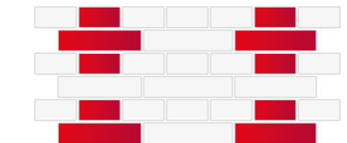
CROSS BINDING TYPE 1
